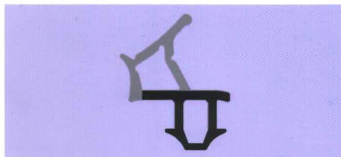
3000 zendow MULTIFUNCTIONAL WEATHERSEAL
